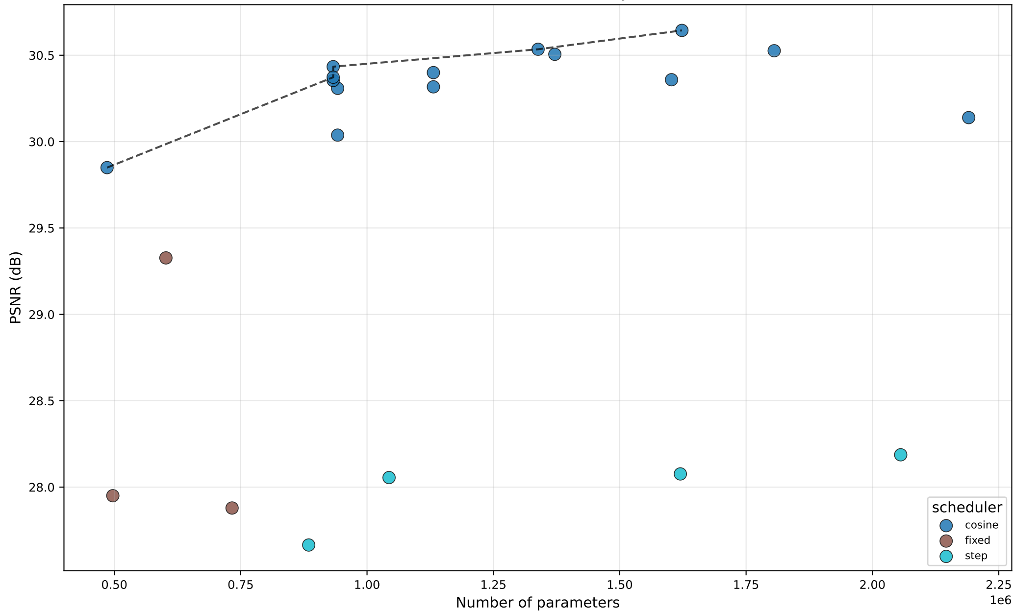
PSNR vs #Params — ELAN — by scheduler
